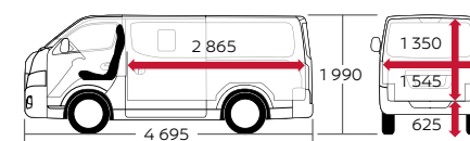
Panel Van Standard Body, Standard Roof
